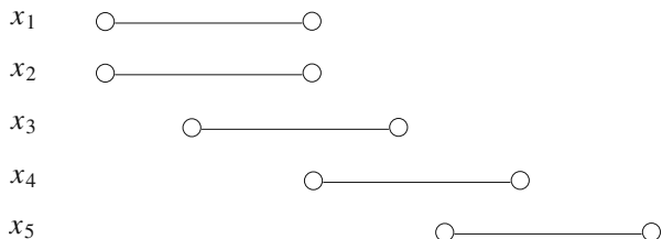
Fig. 1 Example of abstract interval ordering
