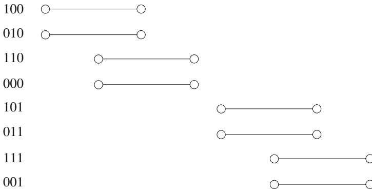
Fig. 3 Example of abstract interval ordering
