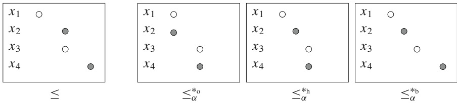
Fig. 4 An initial tpo \leq and the result of revising \leq by \alpha using *_o , *_h and *_b resp., where [\alpha] = \{x_2, x_4\}
